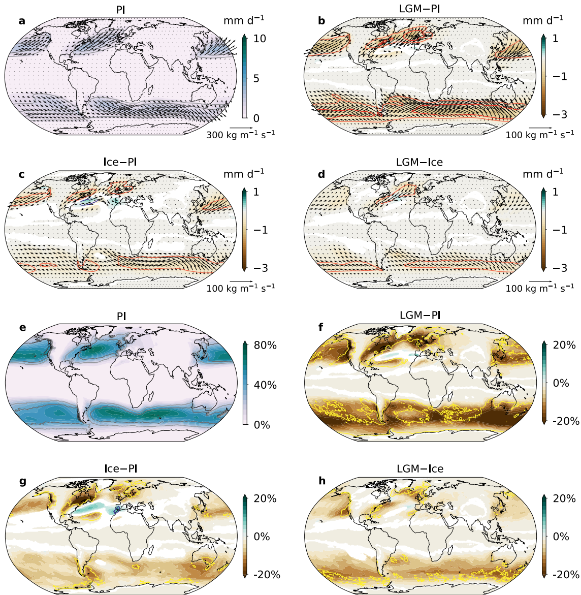
Figure 3. Atmospheric rivers (ARs). (a–d) Average frequency of AR occurrence (open contours; units are percentage of time steps with AR conditions; 10%, 20%, and 30% contours are shown in panel (a), and –10%, –5%, 5%, and 10% contours, from red to blue, in panels (b)–(d)), atmospheric moisture transport due to ARs (arrows), and precipitation associated with ARs (filled contours). Panels as in Figures 1a–1d. (e–h) Average percentage of total precipitation associated with ARs (filled contours) and average percentage of 99th percentile precipitation associated with ARs (open contours; 50%, 70%, and 90% contours are shown in panel (e), –15% (yellow) and +15% (blue) contours shown in panels (f)–(h)). Panels as in (a)–(d).
