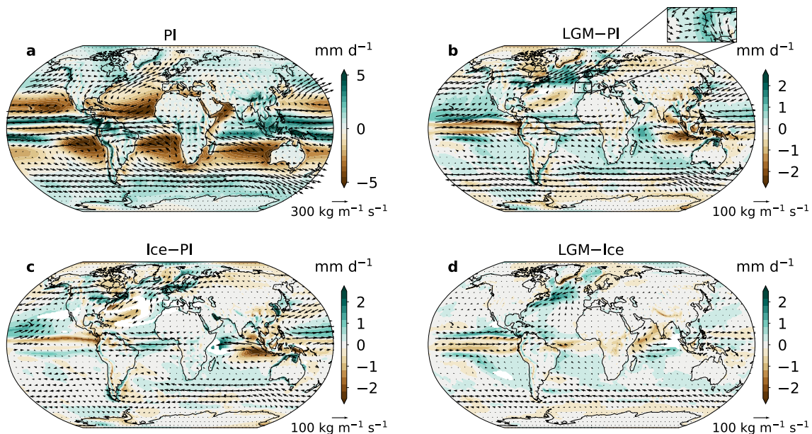
Figure 2. Atmospheric moisture transport and its convergence. Average atmospheric integrated vapor transport (IVT; arrows) and IVT convergence (filled contours). Panels as in Figures 1a–1d. In the inset (panel b), IVT arrows are enlarged by a factor of four relative to the key.
